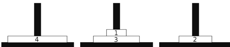
Figure 2. — The configuration 1210 for the Hanoi Towers with four disks
