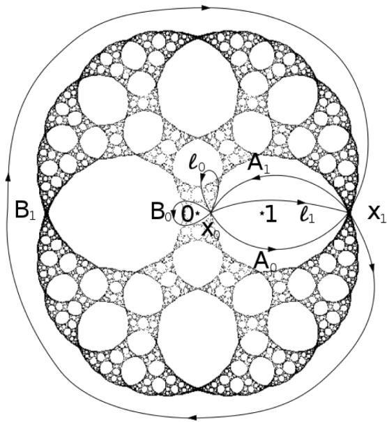
Figure 6. — The labeling choice \ell_0, \ell_1 and the lifts of a, b a, b
