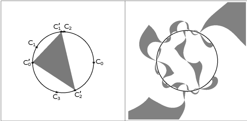
Figure 12. — The loop b_2.b_1.b_0 and its W^5 -lift
