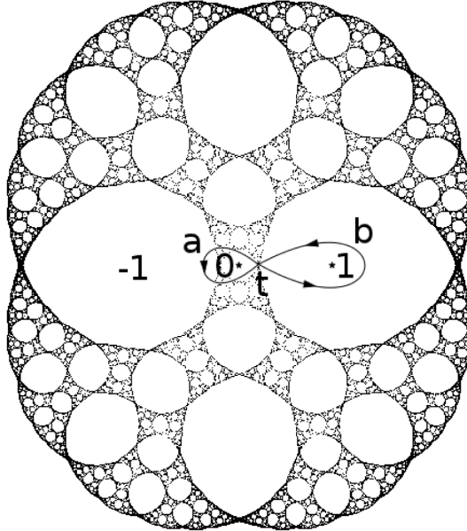
Figure 5. — The Julia set of R : z \mapsto \left(\frac{z-1}{z+1}\right)^2 and two generators of \pi_1(\mathbb{C} \setminus \{0, 1\}, t) a, b
