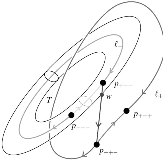
Figure 1. — Flowlines for case C_3 .
