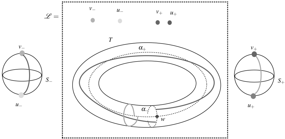
Figure 2. — Non-Hausdorff surface \mathcal{L} for case C_3
