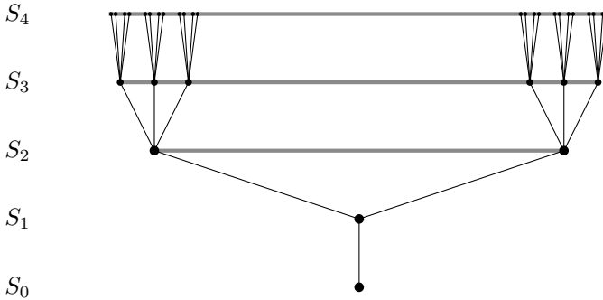
Figure 1. — Growing tree with complete graph on spheres
