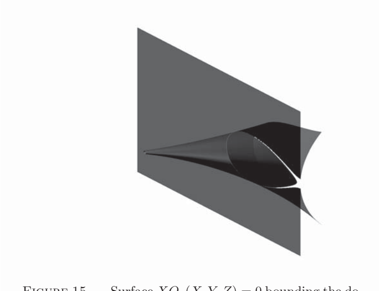
FIGURE 15. — Surface XQ_3(X, Y, Z) = 0 bounding the domain \Omega_{14}
