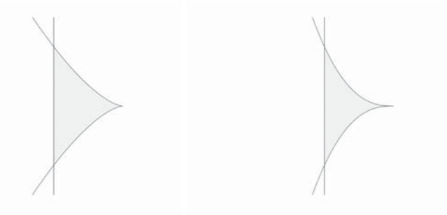
FIGURE 4. — The domains \Omega_3^{(3)} and \Omega_3^{(5)} (for \mathcal{C}_{3,J} and \mathcal{C}_{5,J} )
