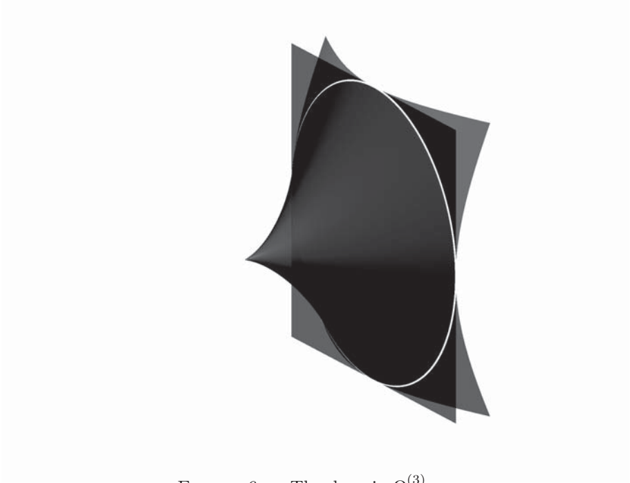
FIGURE 6. — The domain \Omega_4^{(3)}
