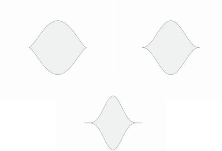
FIGURE 1. — \Omega_1^{(3)}, \Omega_1^{(5)} and \Omega_1^{(11)} .
