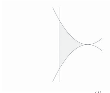
FIGURE 5. — The domain \Omega_3^{(4)}
