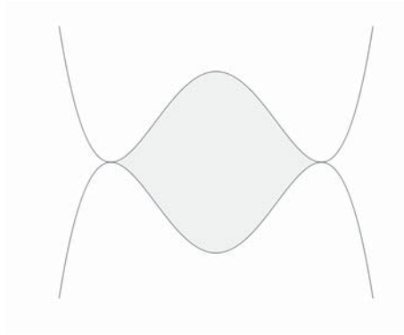
FIGURE 2. — \Omega_1^{(4)} to illustrate the even case
