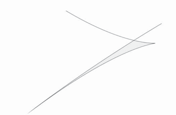
FIGURE 17. — Domain \Omega_{21} bounded by S(X, Y) = 0 .
