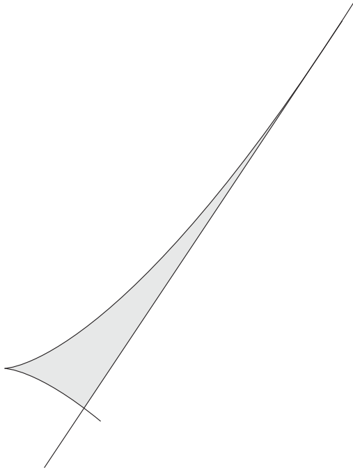
FIGURE 14. — The domain \Omega_{13} : cuspidal cubic with tangent.
