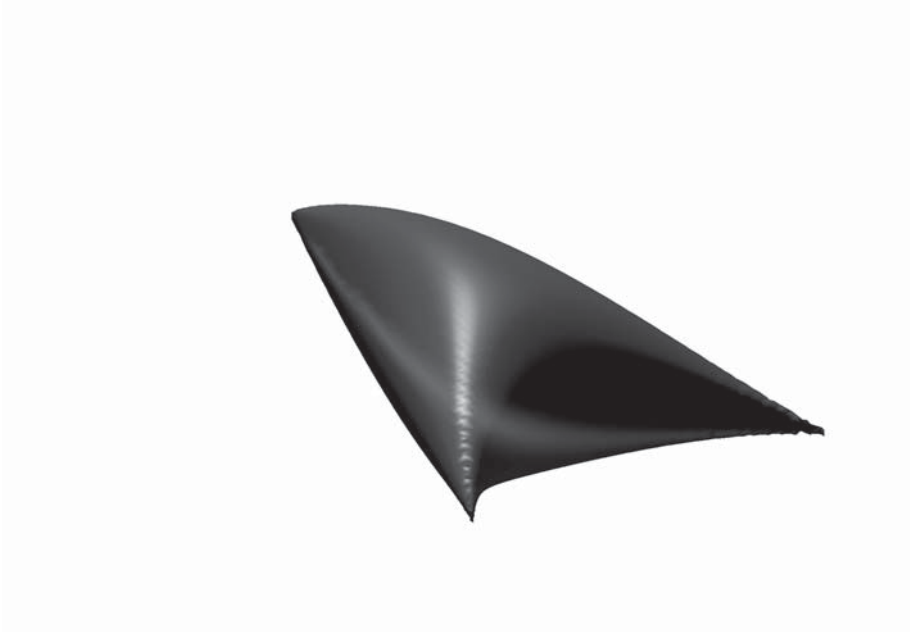
FIGURE 13. — Surface P_3(X, Y, Z) = 0 , bounding \Omega_{12} .
