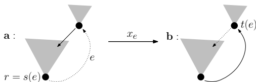
Figure 2.1. An edge \mathbf{a} \rightarrow \mathbf{b} in the tree graph \mathcal{T}G . It is associated with the edge weight x_e .
