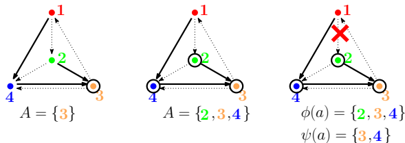
Figure 3.1. Left: in plain edges, a spanning tree \mathbf{a} of the graph of Figure 1.1. We initialize the set A to \{3\} since 3 is the root of \mathbf{a} . Center: at the first two iterations of the main loop of the algorithm, we consider the edges (2, 3) and (4, 3) , that belong to the tree \mathbf{a} : the vertices 2 and 4 are thus added to the set A . Right: at the next iteration, we consider the edge (1, 2) that does not belong to \mathbf{a} . The vertex 1 is thus erased. The set A will not evolve until the termination step, and we thus get \phi(\mathbf{a}) = \{2, 3, 4\} . The strongly connected component of 3 inside \{2, 3, 4\} in the original graph is \{3, 4\} , which gives the value of \psi(\mathbf{a}) .
