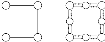
Figure 6.1. Left: The hypercube \{0, 1\}^2 ; Right: the graph \mathcal{TB} for k = 2 and n_1 = n_2 = 2 .
