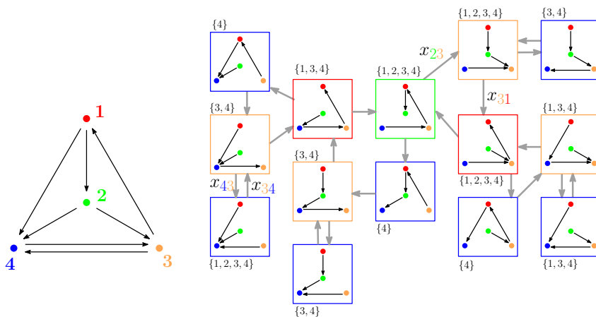
Figure 1.1. A directed graph G with 4 vertices (Left), and the graph \mathcal{T}G (Right). Each vertex of \mathcal{T}G is one of the 14 spanning trees of G . The weight of an edge in \mathcal{T}G only depends on the root vertex of the two trees it links – only certain edge weights are indicated on this picture. The subset of vertices indicated next to each spanning tree is the \psi -value returned by the algorithm of Section 3.2.
