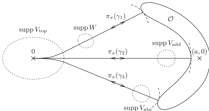
Figure 2.3. A realization with a potential V_{\text{top}} and an obstacle O .
