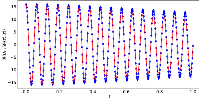
Figure A.1. Real part of U_{k,t}(\phi_t(z), z) for k = 100 and z = p + iq with (p, q) = (0.3, 0.1) , for 0 \leq t \leq 1 .
