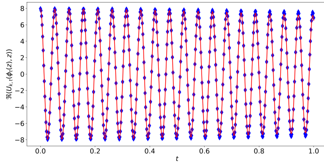
Figure A.3. Real part of U_{k,t}(\phi_t(z), z) for k = 50 and z = p + iq with (p, q) = (0.5, 0.7) , for 0 \leq t \leq 1 .
