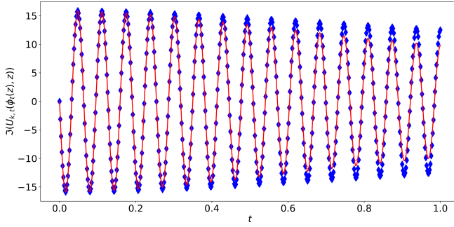
Figure A.2. Imaginary part of U_{k,t}(\phi_t(z), z) for k = 100 and z = p + iq with (p, q) = (0.3, 0.1) , for 0 \leq t \leq 1 .
