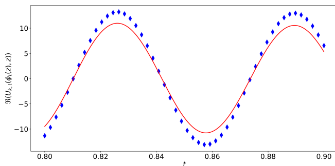
Figure A.5. Real part of U_{k,t}(\phi_t(z), z) for k = 100 and z = p + iq with (p, q) = (0.3, 0.1) , for 0.8 \leq t \leq 0.9 .
