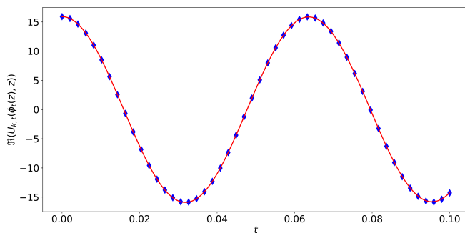
Figure A.4. Real part of U_{k,t}(\phi_t(z), z) for k = 100 and z = p + iq with (p, q) = (0.3, 0.1) , for 0 \leq t \leq 0.1 .
